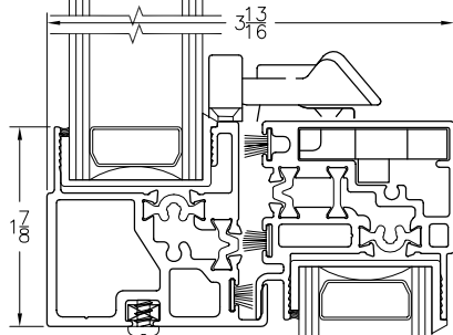
2 MEETING RAIL
