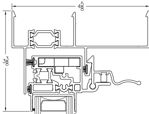
1 HEAD
