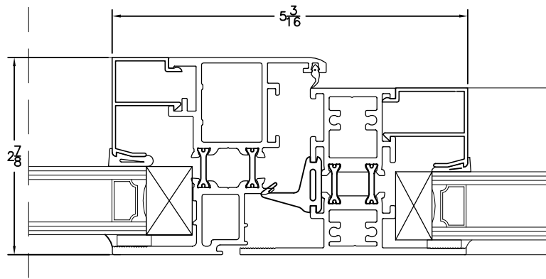
8 OPER/FX MULLION
