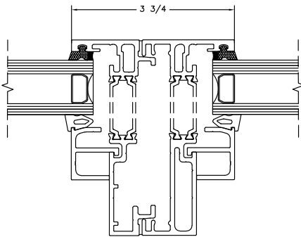
FIXED/FIXED STACKED MULLION
