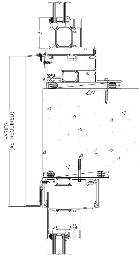
METAL SLAB EDGE COVER
