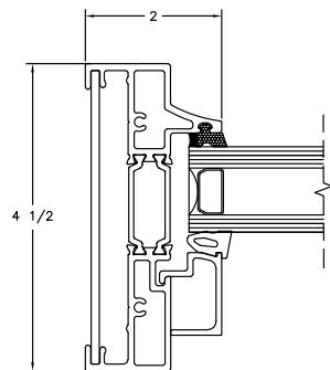
FIXED JAMB ALTERNATE FRAME DESIGN
