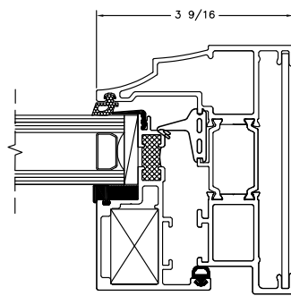
OPERABLE JAMB ALTERNATE FRAME DESIGN
